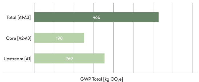
Hot-rolled merchant bar - Vicenza [kg CO 2 e]
