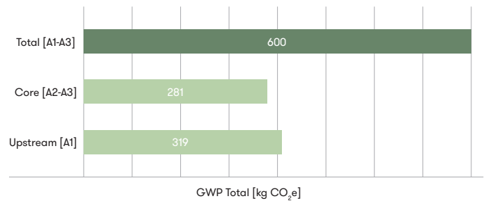
Hot-rolled merchant bar - San Giovanni Valdarno [kg CO 2 e]
